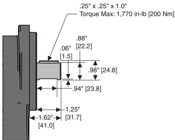
Product Code M1 – SAE “B” Key Parallel
